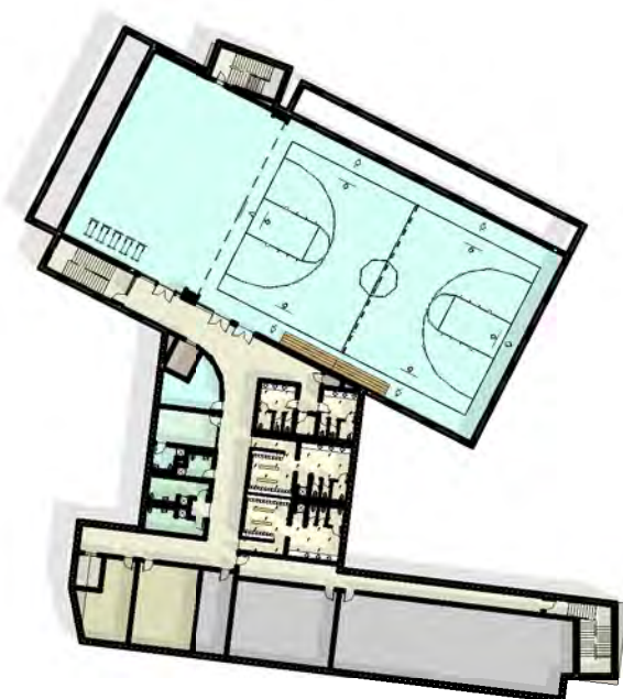
PLAN - GYM FLOOR
